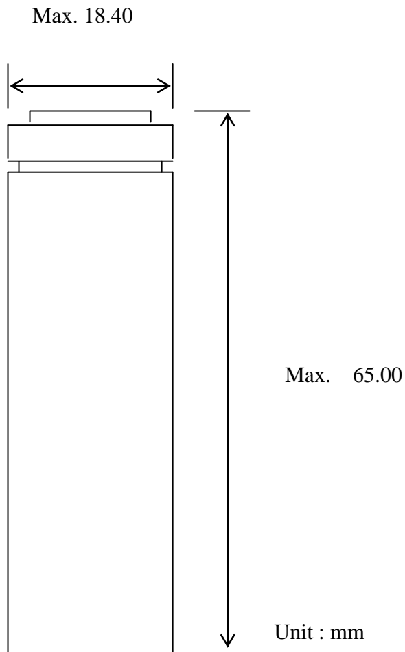
Fig.1. Outline Dimensions of ICR18650-28A (with Tube)
