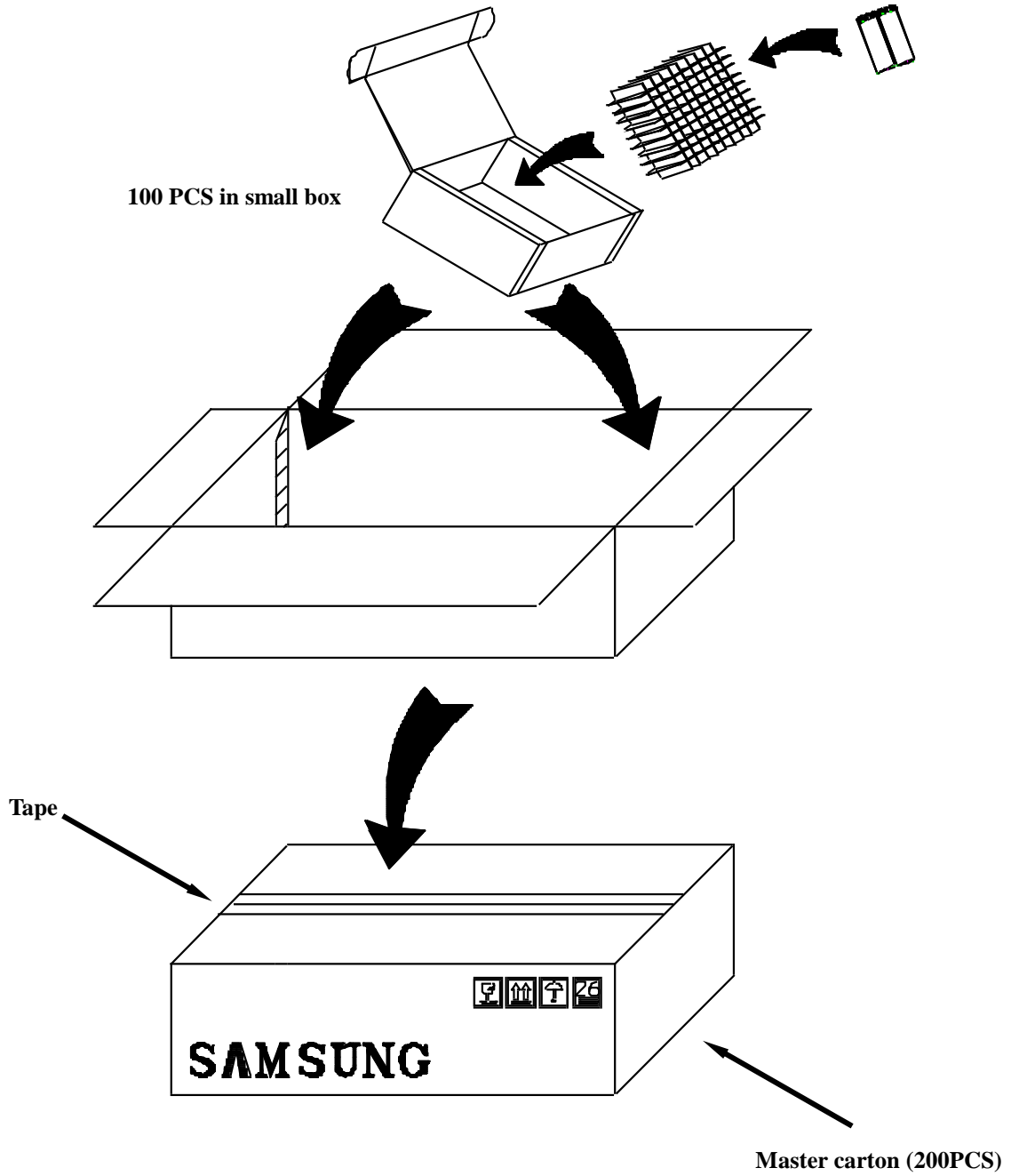
Fig.2. Package Drawing
